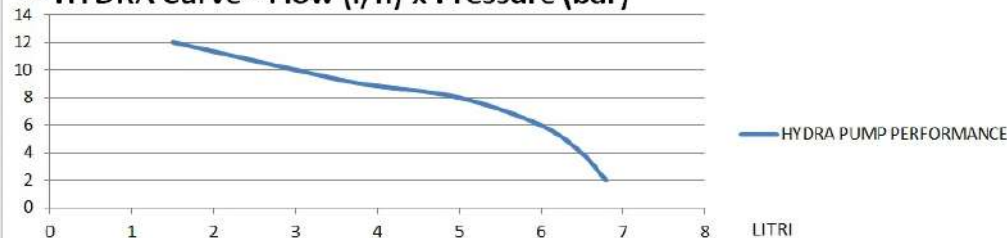
HYDRA Curve - Flow (l/h) x Pressure (bar)
